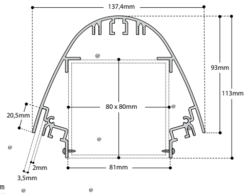
Aluminium or steel profile 80 x 80 x 4mm Aluminium- eller stålprofil 80 x 80 x 4mm
